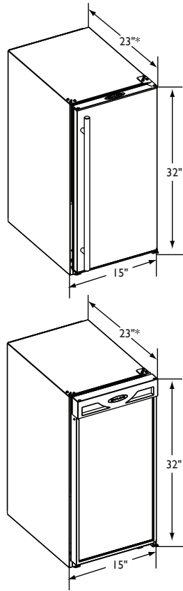
ADA151MS Stainless Model and ADA151MB Black Model * Add 3/4" for water line clearance
